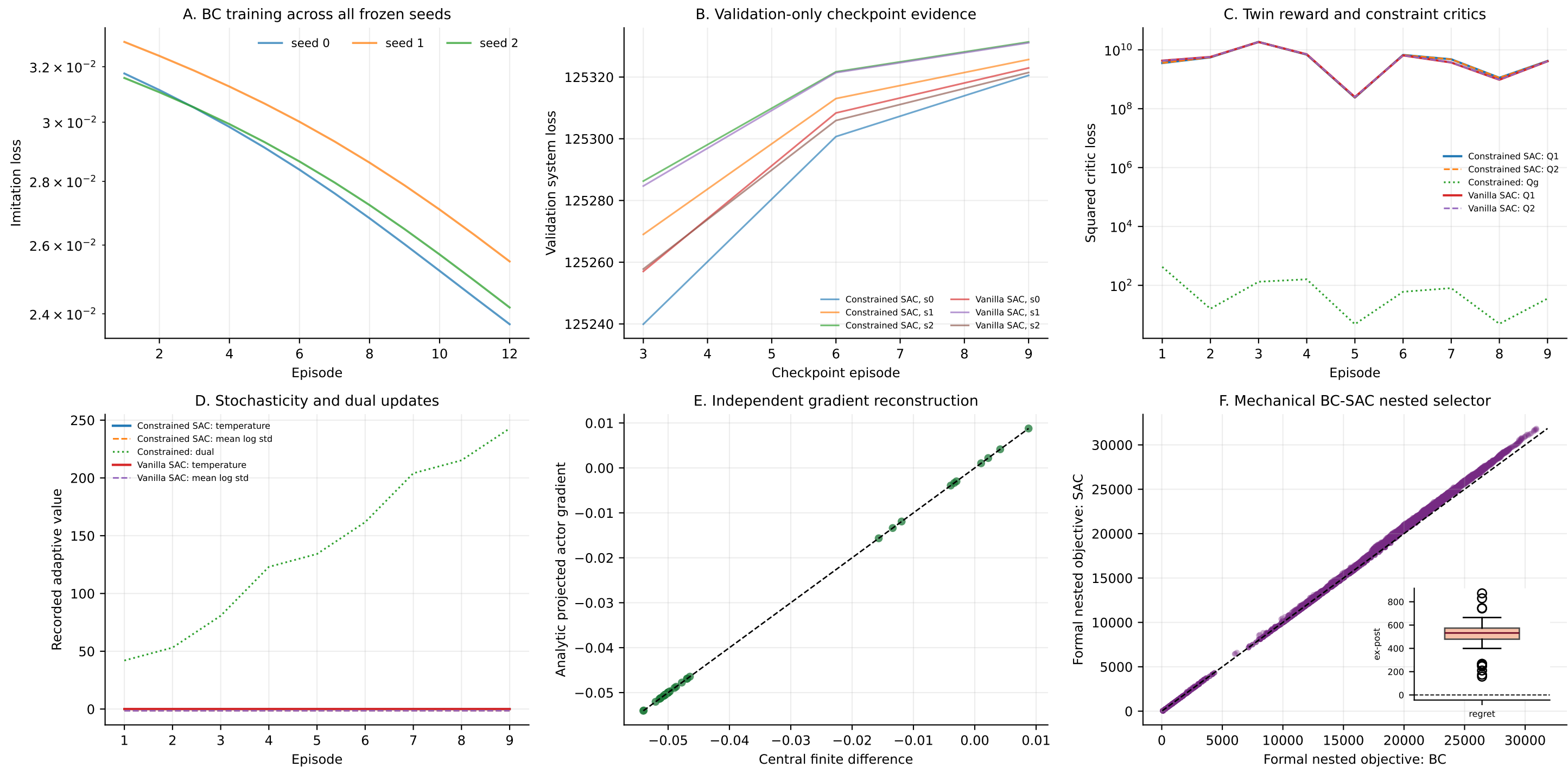
Figure 5.2.5b Learning and selector acceptance
